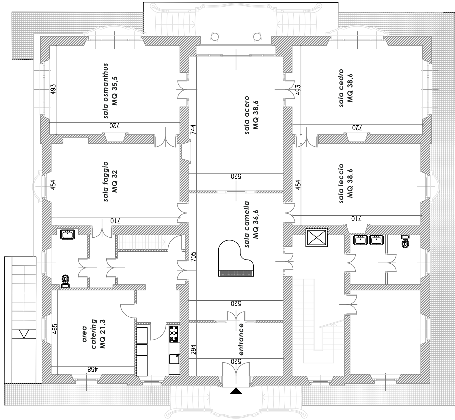
pianta piano rialzato | ground floor map
