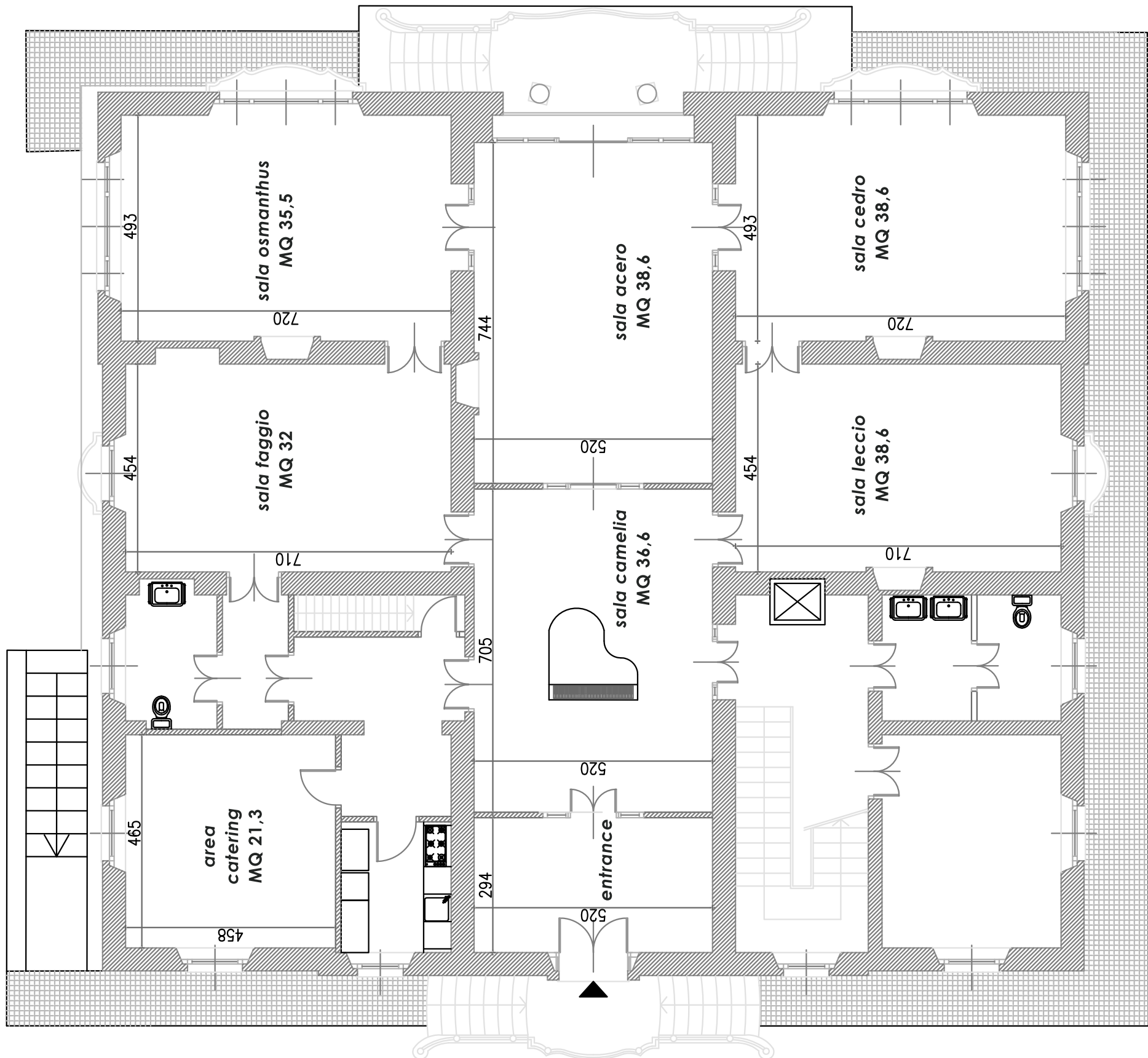
pianta piano rialzato | ground floor map
